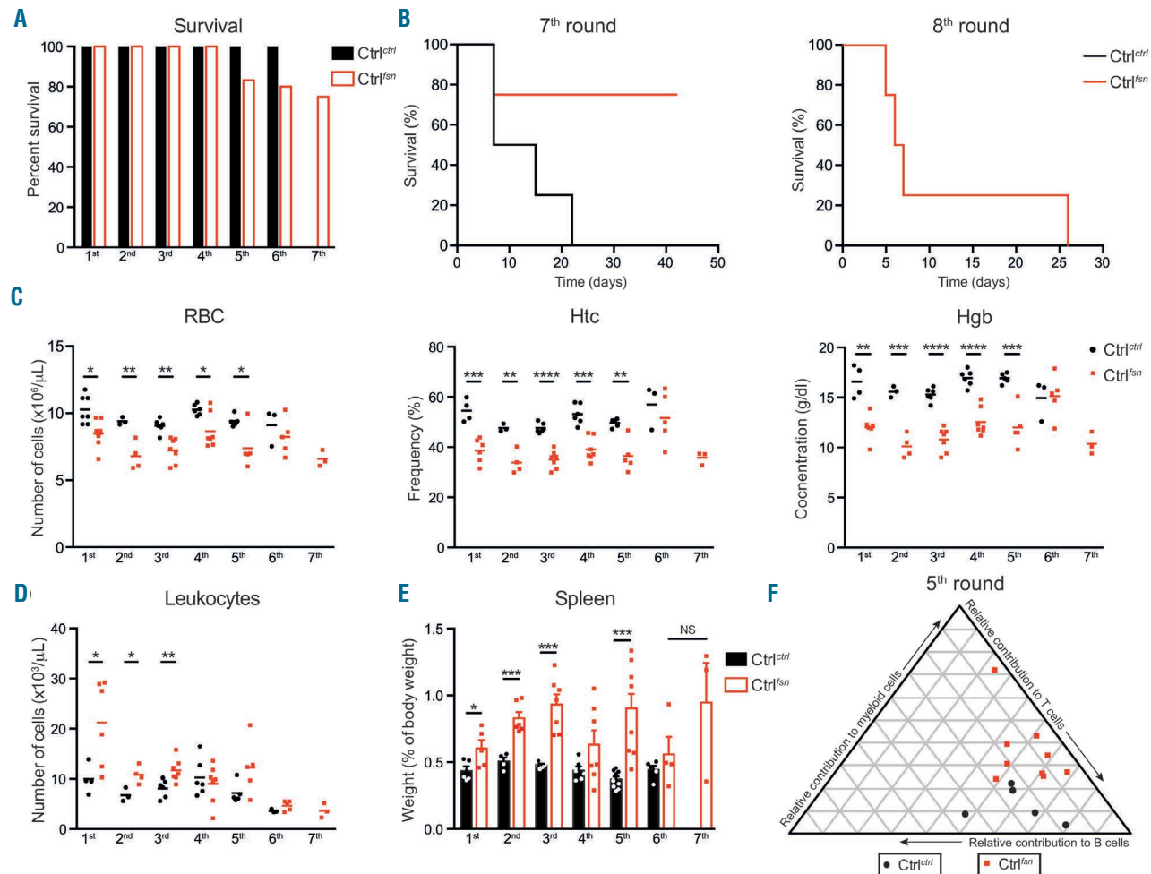
Figure 5. Ttc7a -deficiency promotes self-renewal ability of hematopoietic stem cells. Lethally irradiated mice were serially transplanted with 3-week old ctrl ( Ctrl ctrl – black bars, dots and lines) or Ttc7a -deficient ( Ctrl fln – red bars, dots and lines) donor bone marrow (BM) cells (mean \pm standard error of mean) *P < 0.05 ; **P < 0.01 ; ***P < 0.001 ; ****P < 0.0001 (two-tailed t -test). These data are representative of four independent experiments with at least four mice in each round of transplantation. (A) Percent survival of recipient mice across the seven transplantation cycles. (B) Survival of Ctrl ctrl and Ctrl fln mice during the seventh round and Ctrl fln mice during the eighth round over time ( n=4 for control- and n=10 for Ttc7a -reconstituted mice). (C-F) Red blood cell count, hematocrit, and hemoglobin level (C), leukocytes count (D) and spleen weight (E) across the transplantation cycles. (F) Relative contribution of myeloid compared to T- and B-lymphoid cells in the spleen of mice transplanted with BM cells that had undergone five transplantation cycles. RBC: red blood cells; Htc: hematocrit; Hgb: hemoglobin.
