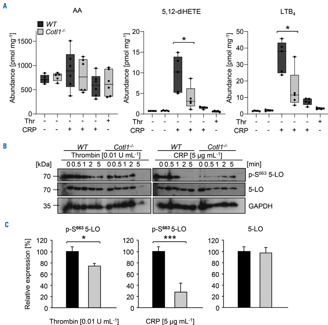
Figure 3. Cott1 is a regulator of leukotriene biosynthesis in platelets. (A) For lipid mediator analysis platelets were either left untreated or stimulated with CRP [5 μg mL -1 ] or thrombin [0.01 U mL -1 ] for 5 minutes (min). Subsequently, samples were spun down, pellet and supernatant were separately shock-frozen in liquid nitrogen. Lipid abundance was assessed using liquid crystal mass spectrometry. Values are mean±standard deviation (SD) (n=15). (B and C) Platelets were either left untreated or stimulated with CRP [5 μg mL -1 ] or thrombin [0.01 U mL -1 ] for 5 min, lysed, and processed for immunoblotting. Total 5-LO, phospho-5-LO (S663) and GAPDH (B) were probed with the respective antibodies and analyzed by densitometry (C). Values are mean±SD (n=4).
