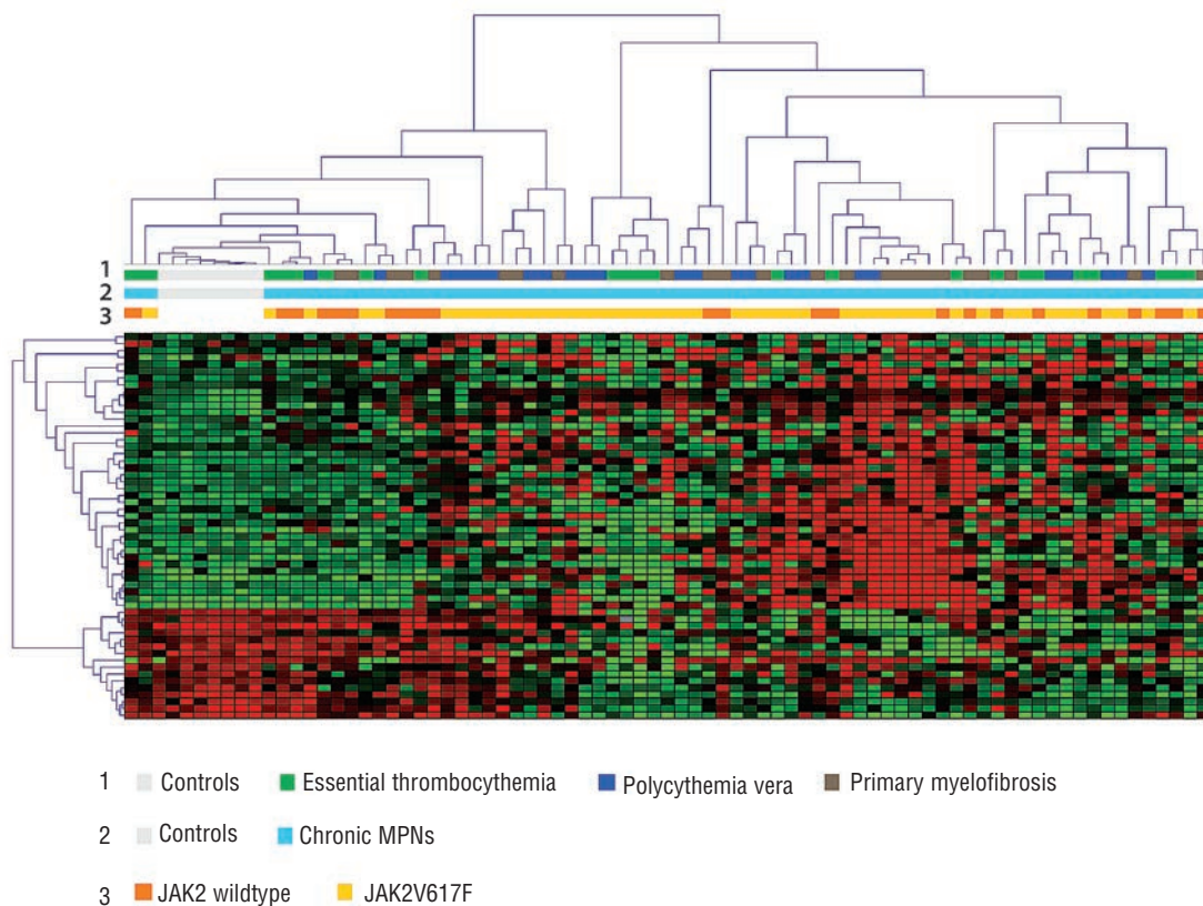
Figure 1. Hierarchical cluster analysis based on differentially methylated genes in MPNs samples in comparison with healthy donor samples. \beta values are depicted using a pseudocolor scale. Red: hypermethylated genes; Green: unmethylated genes. The top bar beneath the dendrogram indicates PV, ET, PMF sample type in a specific color-code. Second bar indicates MPNs and healthy donor samples. Third bar indicates MPNs samples with or without JAK2V617F mutation.
