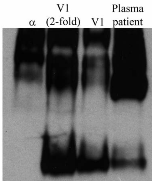
Online Supplementary Figure S2. Western blotting of purified mutant V1 and antithrombin from plasma of the patient run on native PAGE with urea.
