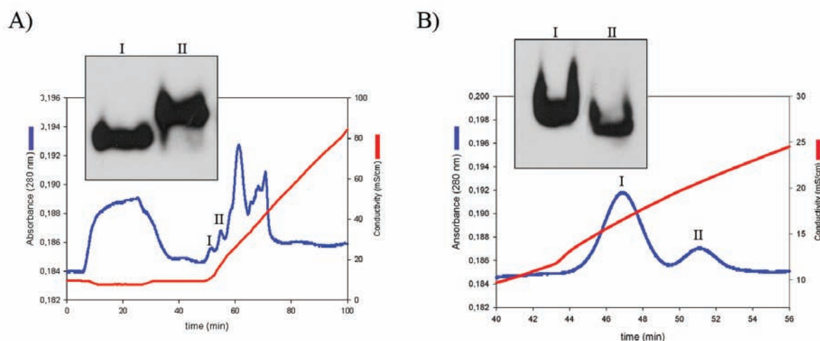
Online Supplementary Figure S1. Anion exchange chromatography profiles and Western blotting of native gels of purified mutant variants. (A) Purification of V1 from the first peak obtained by heparin sepharose chromatography from the plasma of the patient, where the wild-type latent form also eluted. (B) Purification of V2 from the second peak obtained by heparin sepharose chromatography from the plasma of the patient, where the wild-type \alpha isoform also eluted.
