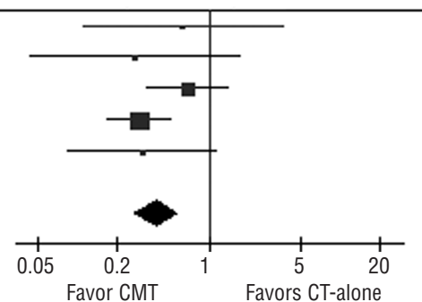
Figure 3. Meta-analysis of OS among patients with early stage Hodgkin's lymphoma, who received chemotherapy (CT) alone or chemotherapy and radiotherapy (CMT). Solid squares represent effect estimates for the single trials, the size of square represents the weight of individual studies in the meta-analysis. Horizontal lines indicate 95% confidence intervals (CIs). The width of diamonds shows the 95% confidence intervals for the pooled hazard ratios.
