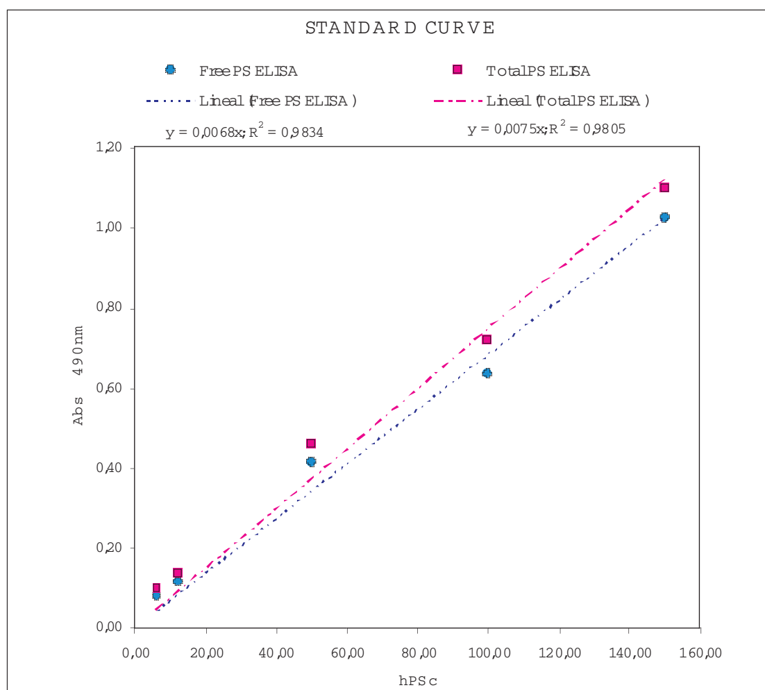
Supplementary Figure S1. Standard curve for PS measurements with the total and free PS ELISA assay. 150, 100, 50, 12.5 and 6.25 ng of purified human plasma PS (hPSc) in phosphate-buffered saline were measured with each assay.
