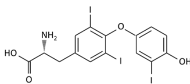
Triiodothyronine (T3)
