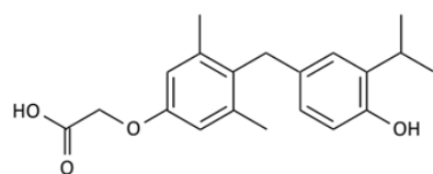
GC-1 (Sobetirome)
