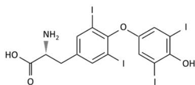
Thyroxine (T4)
