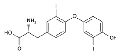
Diiodothyronine (T2)
