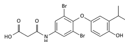
KB2115 (Eprotirome)
