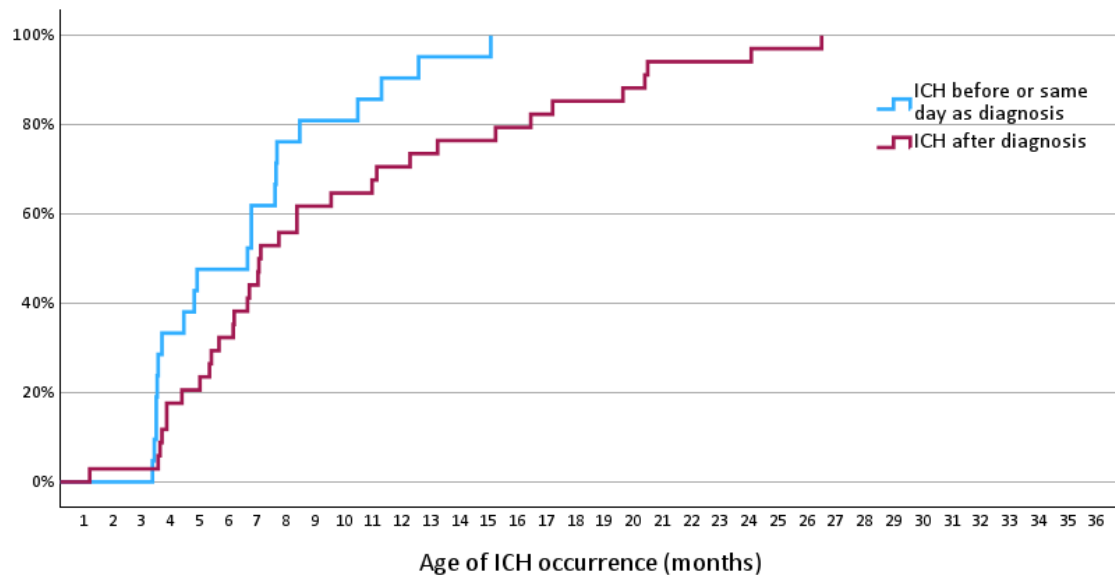
Supplement figure S1: Natural course of ICH: Proportion of all ICH patients with severe hemophilia A and B without prophylaxis: timing of ICH for patients with and without established diagnosis of hemophilia by month of age
