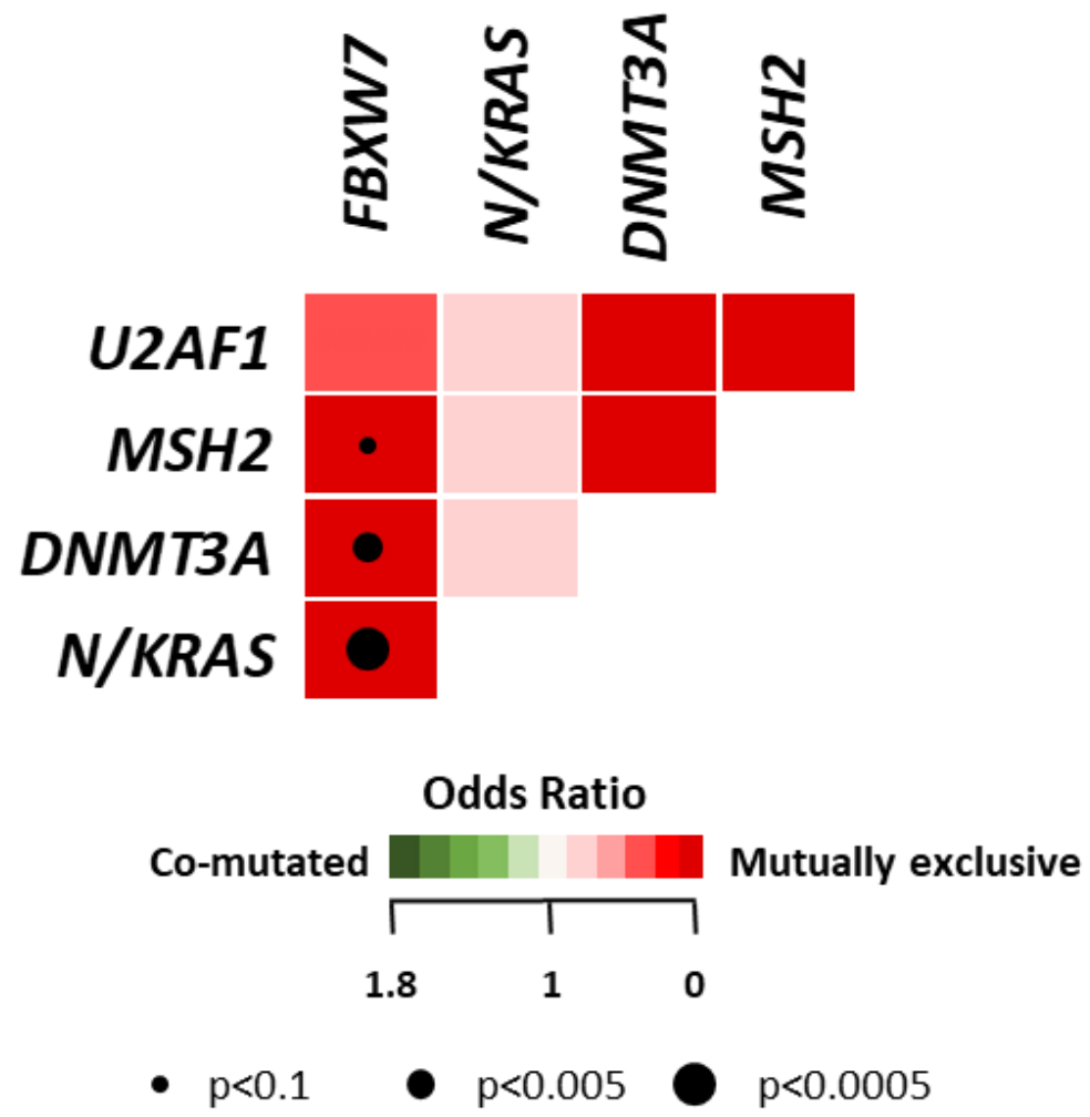
Supplemental Figure 4. Co-occurrence between genes with prognostic impact in the T-ALL cohort. Positive (odds ratio >1) and negative (odds ratio <1) correlations are depicted as green and red, respectively. Black circle diameters indicate the degree of significance.
